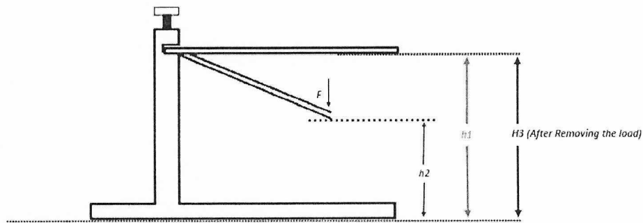
Figure:- 1 Card in Clamping device h1- Before Loading h2- After Loading h3- After Removing the Load
