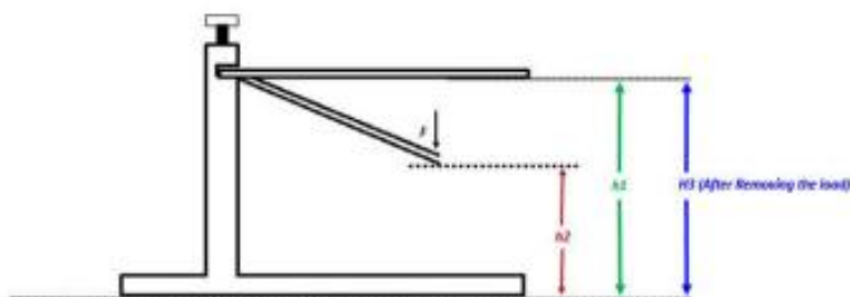
Figure:- 1 Card in Clamping device
